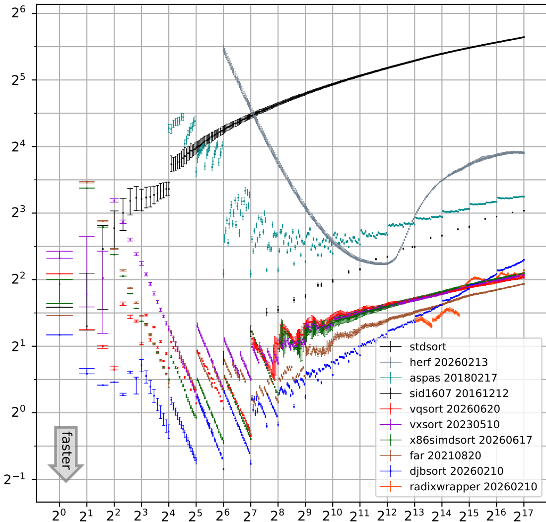
y = \text{cycles/byte to sort int32}[x] on samba (20260621; sortbench-20260621)
