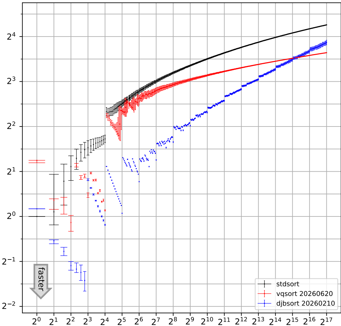
y = cycles/byte to sort int64[x] on pi5 (20260621; sortbench-20260621)
