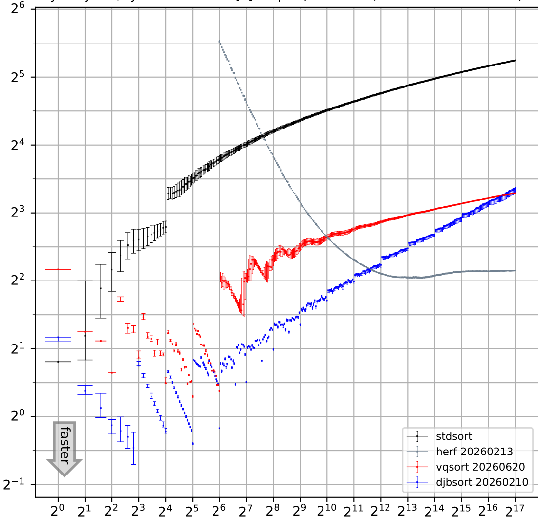
y = cycles/byte to sort int32[x] on pi5 (20260621; sortbench-20260621)
